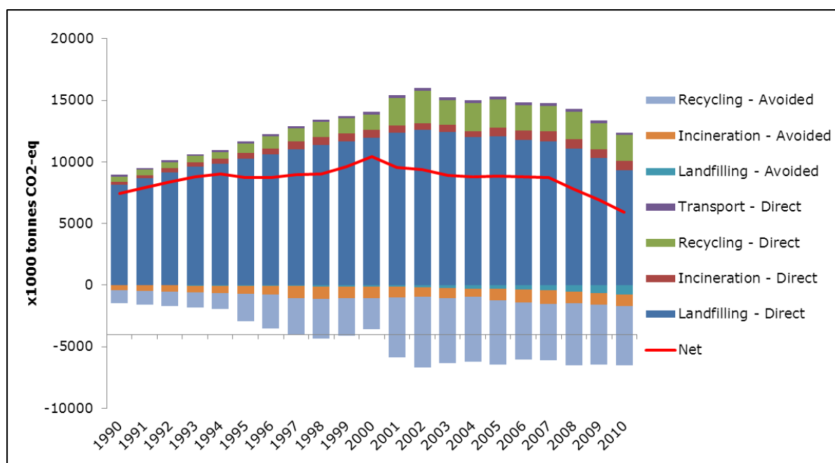
Figure 2.7 GHG emissions from MSW management in Spain
